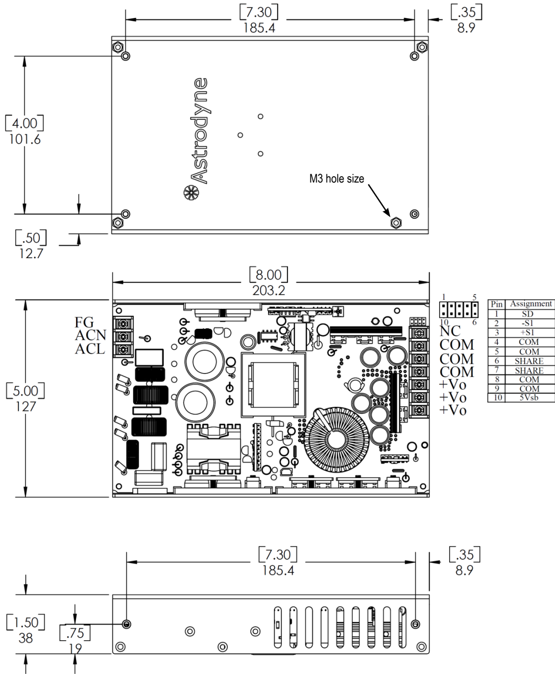
U-Bracket (PMMK450S-xxU)
