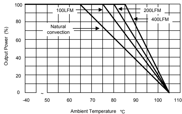
Derating Curve
