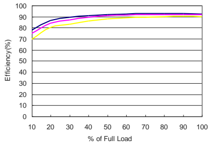
MKW40-24S05 Efficiency vs Load Current
