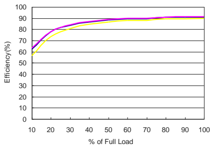
MKW40-24D12 Efficiency vs Load Current
