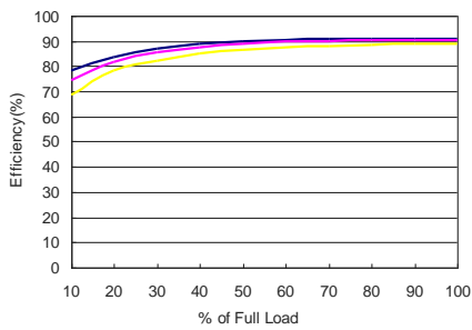
MKW40-24S15 Efficiency vs Load Current
