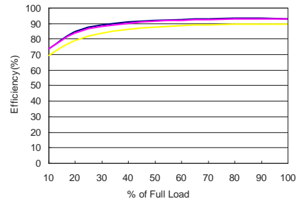
MKW40-24S12 Efficiency vs Load Current
