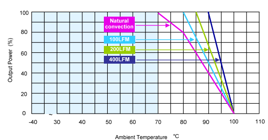
Derating Curve with Heatsink
